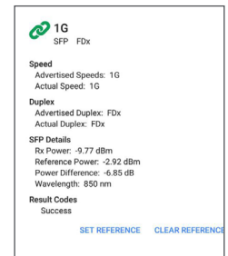
Optical power meter
