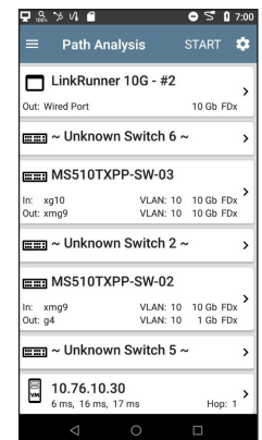
Path Analysis shows the device & interfaces that UDP/TCP traffic traverses
