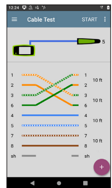
Cable test with Wiremap detecting distance to fault, including cable shield
